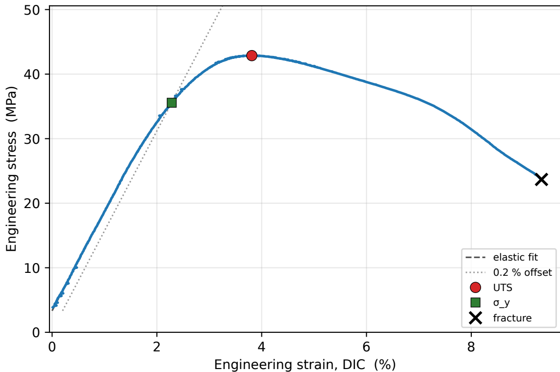
Stress-strain
